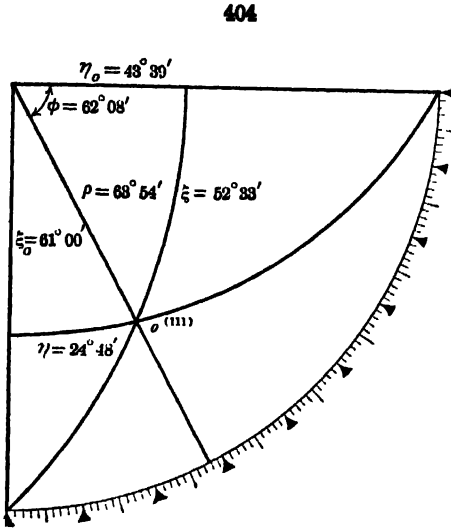
Stereographic Projection of o(111) of Topaz
